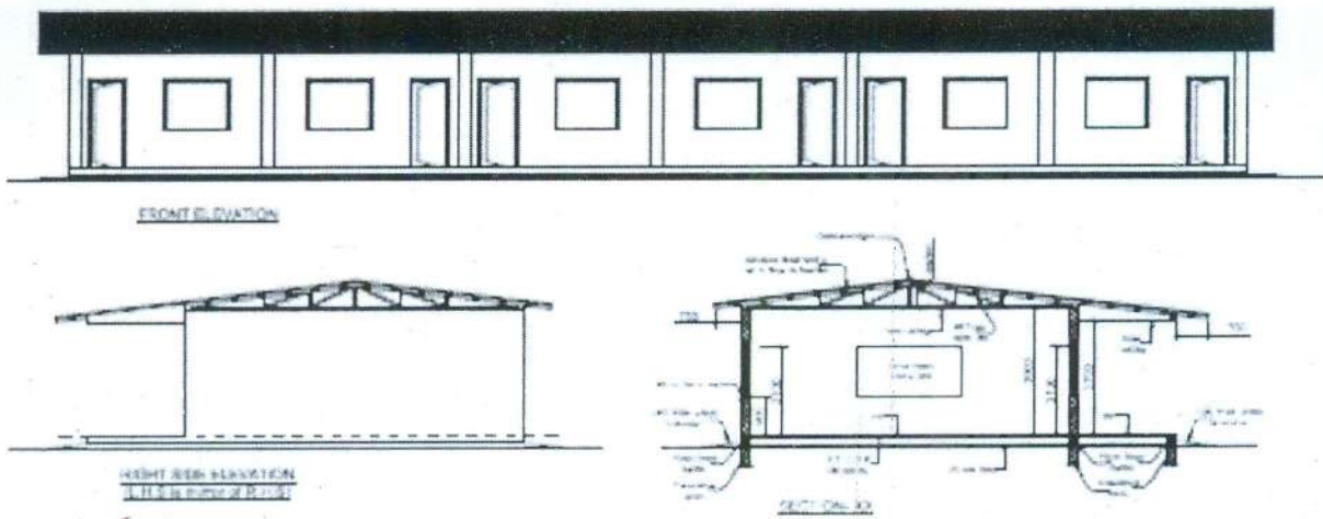
DW-02 ELEVATION & SECTIONS
