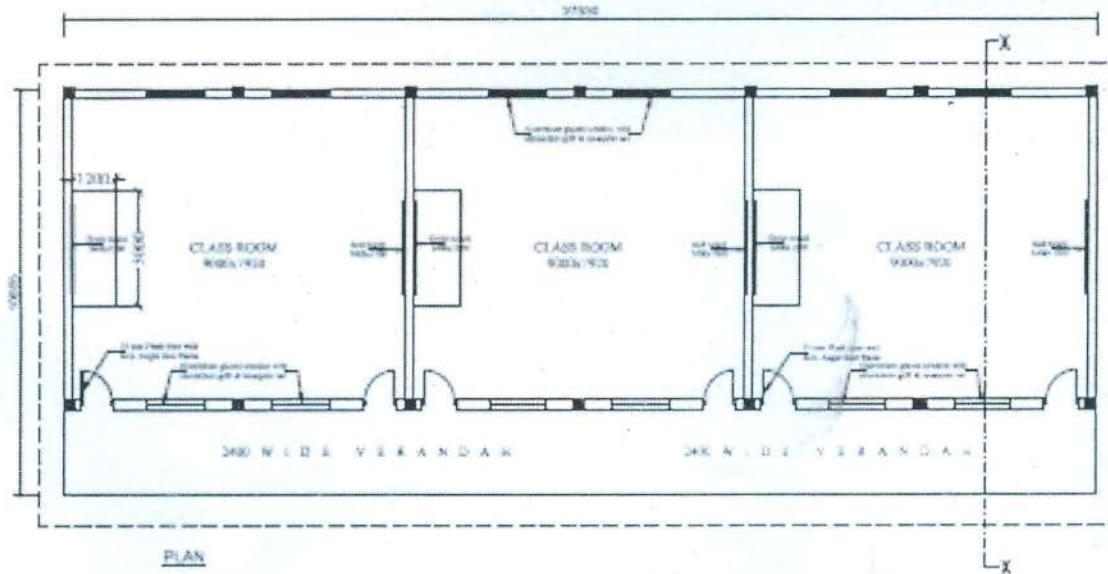
DW-01 PLAN Note: All dimensions in mm
