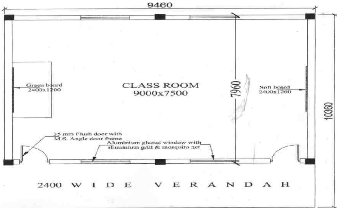
PLAN 1- CR
