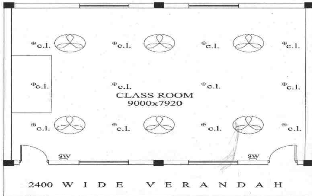
INT. ELECTRIFICATION PLAN FOR 1-CR
