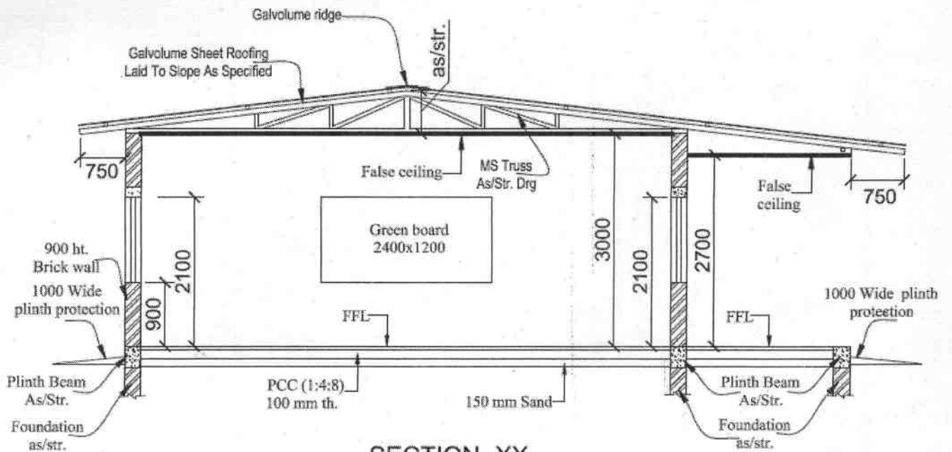
SECTION- XX
